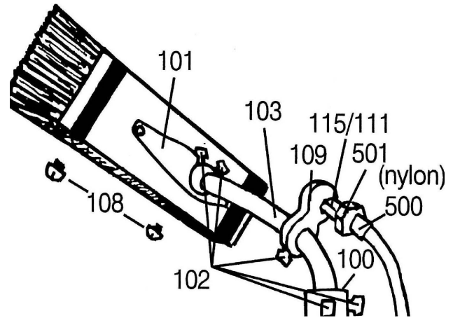
B TYPE DISPENSER
