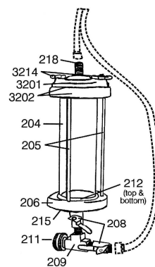
C TYPE DISPENSER
