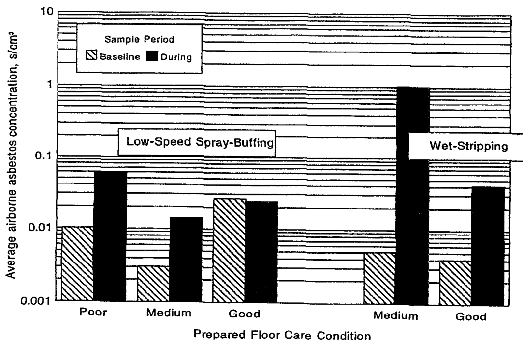
Figure 1. Average airborne asbestos concentrations during low-speed spraying of floors in prepared conditions.
